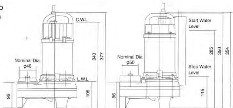
40PU2.15S C.W.L.: Continuous Running Water Level L.W.L.: Lowest Running Water Level
